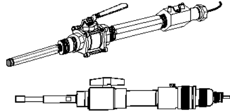
Top: 4909 SS Insertion/Removal Cell Assembly Bottom: 4909 CPVC Plastic Insertion/Removal Cell Assembly
