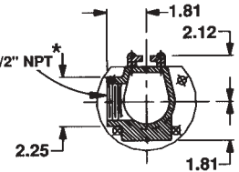
Bossed 3" Back Inlet Section LB-3B, LBA-3B
