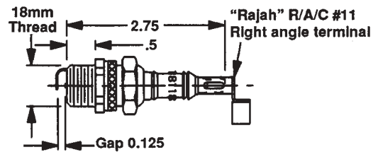
18mm Spark Ignitor
