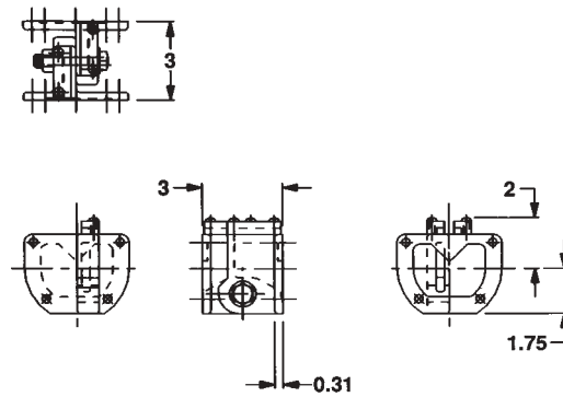
VFL-XEP expansion end plate set
