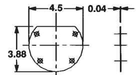
LDP Division Plate
