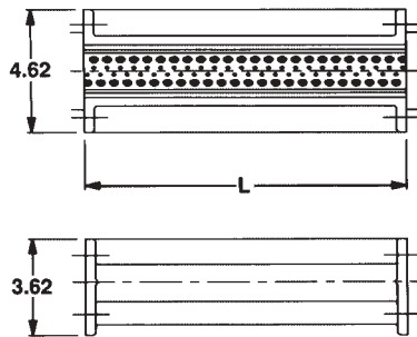
VFH straight sections
