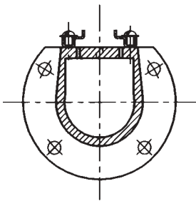
Typical Cross Sectional View of Style A LINOFLAME® Burner with alloy ignition rails
