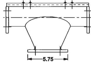
Inlet flange set options for back inlet tee section
