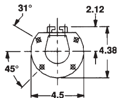
End view typical of all Style B LINOFLAME® Burner straight sections
