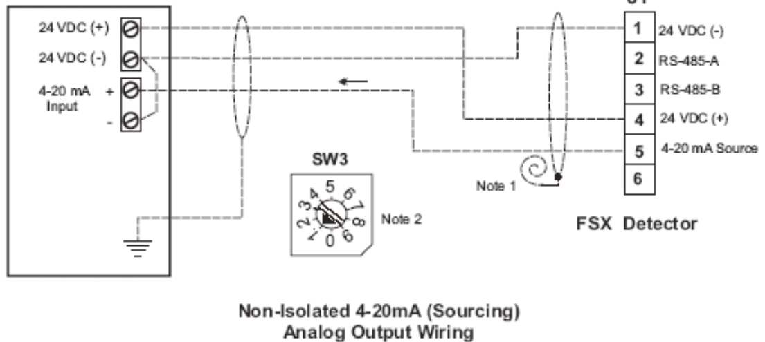
Figure 4-5 Typical Wiring for 4-20mA (Sourcing) Analog Output
