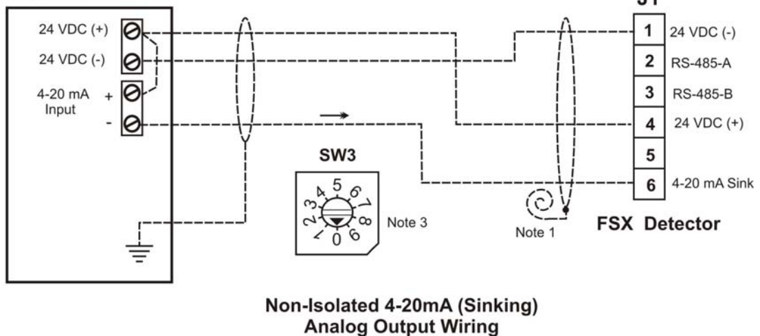
Figure 4-6 Typical Wiring for 4-20mA (Sinking) Analog Output
