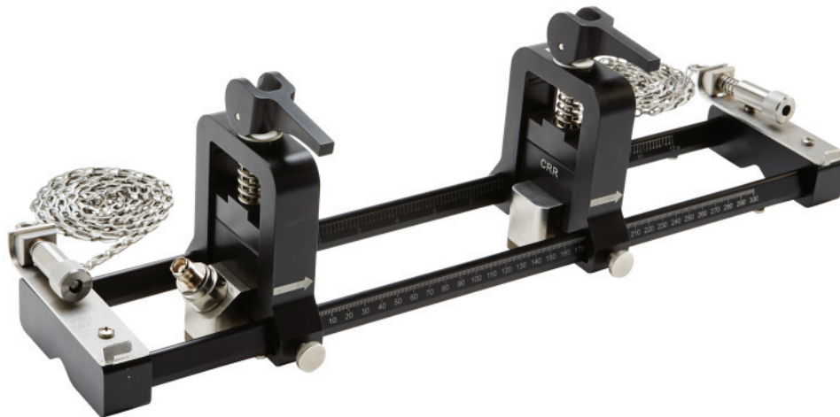
Clamp-On Fixture with CRR Transducers
