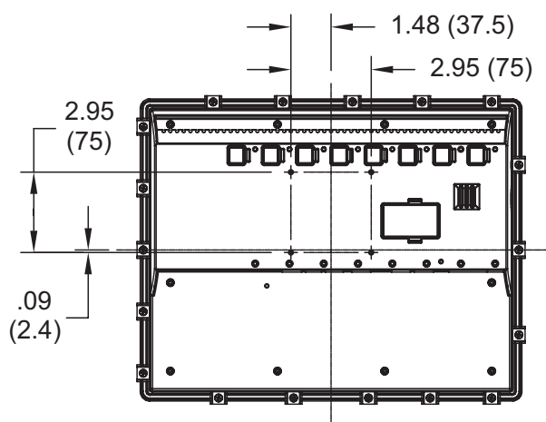
VESA MOUNT (MIS-D 75) DIMENSIONS
