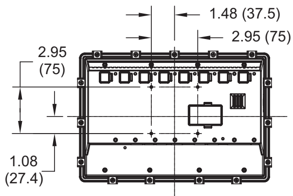
VESA MOUNT (MIS-D 75) DIMENSIONS
