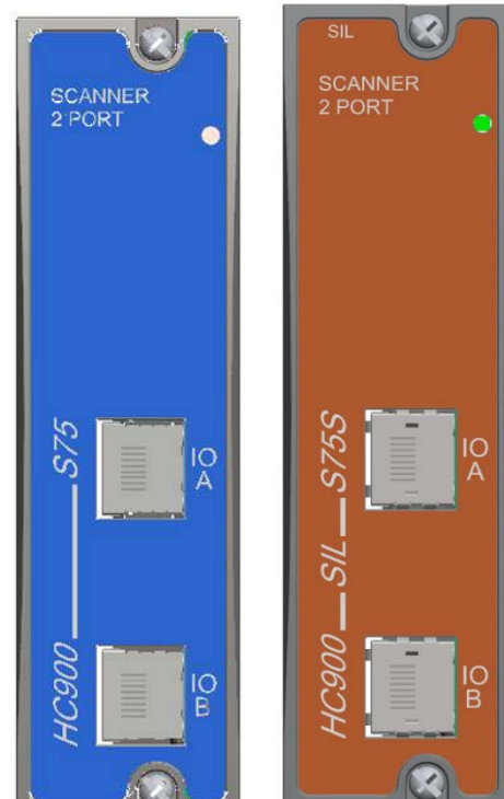
Process Scanner (blue) Safety Scanner (orange)
